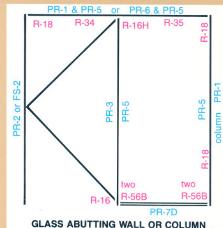
GLASS ABUTTING WALL OR COLUMN
