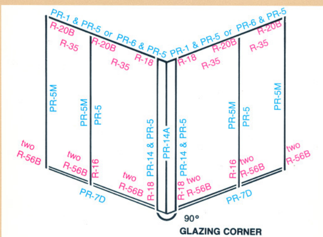
GLAZING CORNER
