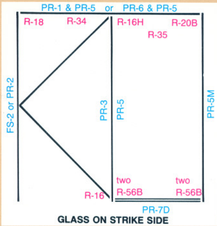
GLASS ON STRIKE SIDE
