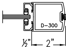
SLIDER NARROW STILE w/ WOOL PILE
