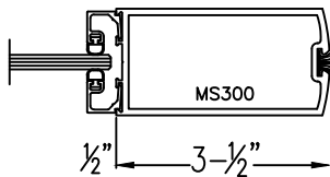
SLIDER MEDIUM STILE w/ WOOL PILE
