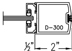
SLIDER NARROW STILE w/ WOOL PILE
